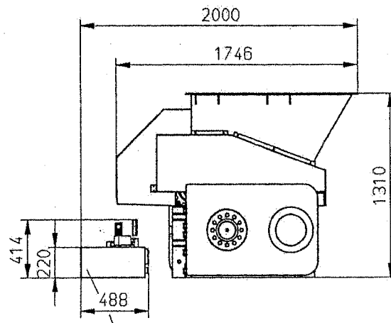
Hydraulikaggregat Lo80-14/8 5,5 Kw Fa. Lotz
